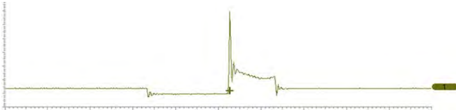
Figure 10-26 Typical Secondary Ignition Signal
