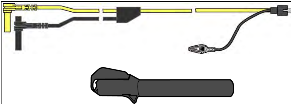
Figure 10-5 Secondary Ignition Coil Adapter Lead and Clip-on Wire Adapter
