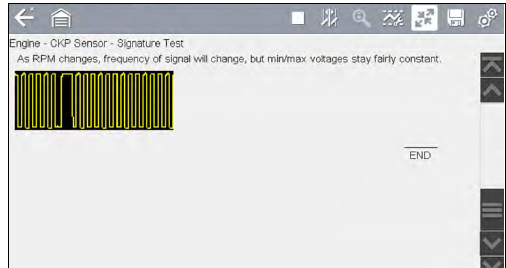
Figure 9-10 Waveform Example
